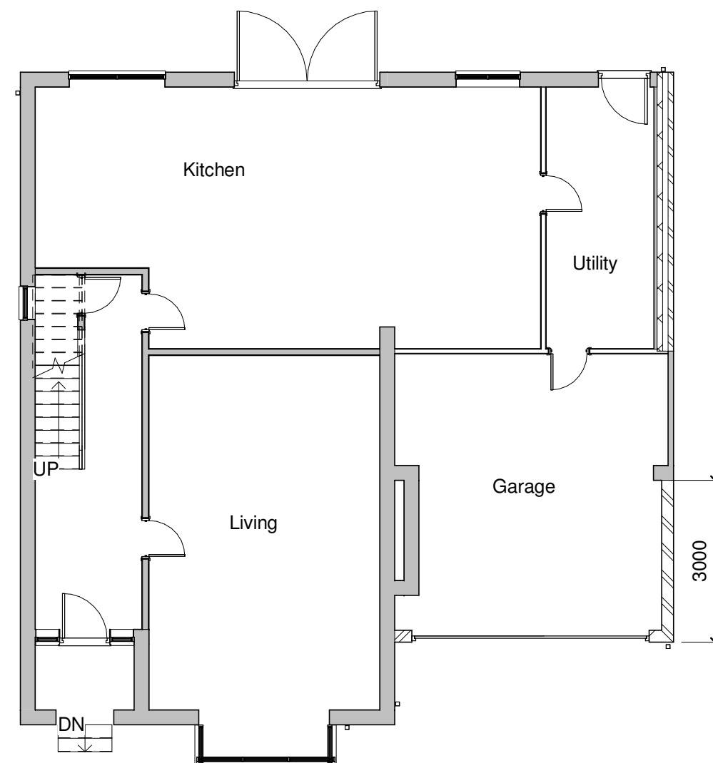
2 Ground Floor 1 : 100
